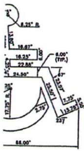
PAVEMENT MARKING SYMBOL
