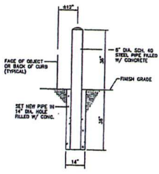
DETAIL BOLLARD NOT TO SCALE
