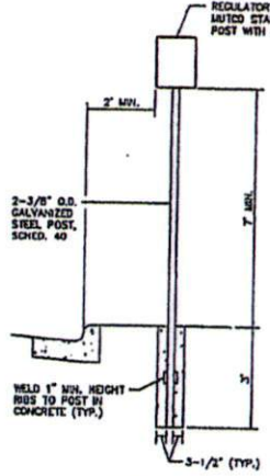
DETAIL SIGN INSTALLATION NOT TO SCALE
